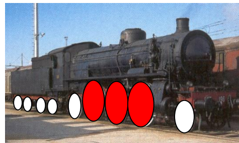
Locomotive + tender
